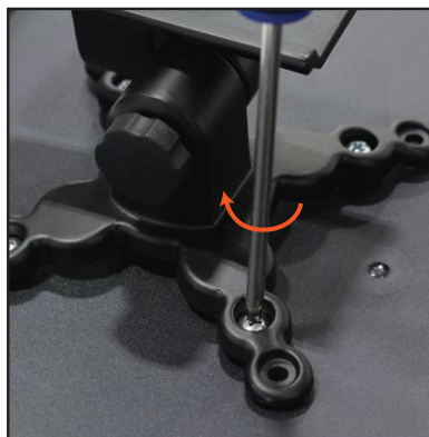
6. Screw monitor bracket to back of monitor. Ensure adjustment knob is facing left is monitor from back.
