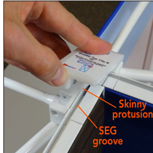
4. Align the skinny protrusion with the SEG groove in the opposite hub.
