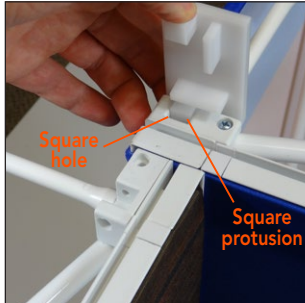
3. Align one square protrusion with the square hole in one hub.
